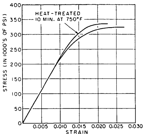
Fig. 2—Tensile stress-strain curves for 0.020 round wire in the as-received condition (lower curve) and after heat-treatment for 10 minutes at 750° F (upper curve).
