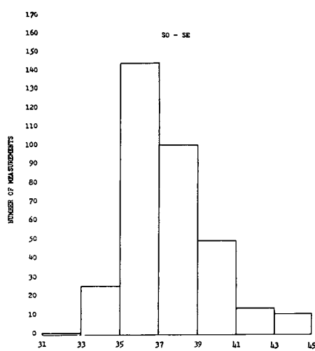
Fig. 3. Frequency distribution of percentage contributed by SO-SE to the total cranial base.
