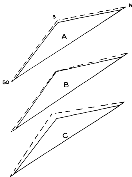
Fig. 14 Possible changes of the Bolton triangle during growth.
