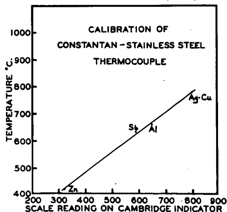
Fig. 2 Graph for conversion of scale readings from constantan-stainless steel thermocouple to degrees centigrade.
