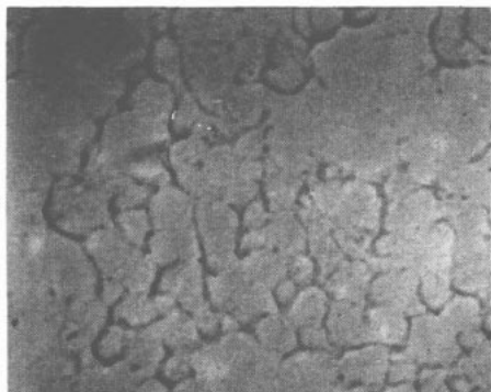
Fig. 6 Electron micrograph of a replica taken from a stainless steel wire heated at 1900° F. for 30 seconds. No carbide particles are present. Note the growth of subgrains. X 26,000
