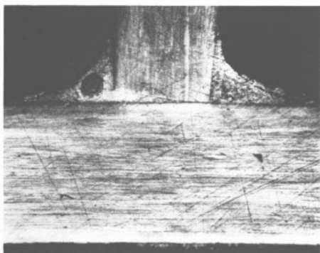
Fig. 7 Soldered union between two stainless steel wires. Void on the left is due to gas inclusion. Note the sharp line of demarcation between solder and steel. X 200
