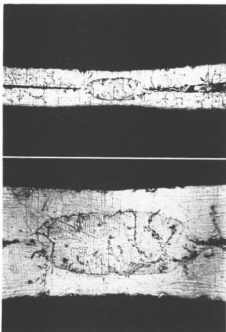
Fig. 4 Above, A proper weld between strips of .003 band material. X 200
