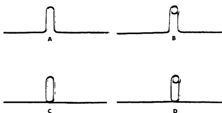
Fig. 1 Wire designs tested: A - open loop; B - helical open loop; C - closed loop; D - helical closed loop.
