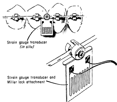
Fig. 12 Transducer assembly modified for electromyographic recording in orthodontic practice.
