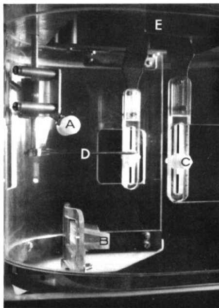
Fig. 1 Cephalostat designed for the Orthopantomograph. A, nasion rest; B, calibrated chin rest; C, calibrated adjustable ear rod assembly; D, infra-orbital marker; E, mechanism to adjust ear rod assembly anteriorly, posteriorly, medially, and laterally.
