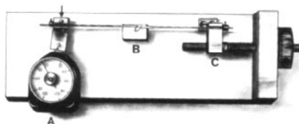
Fig. 2 The calibrating apparatus showing the free ends of the clamp inserted in small holes at the ends of two horizontal rods (B). These rods lie loosely in slots in nylon blocks at either end. The loading is accomplished by means of the screw on the right (C) and recorded on the force gauge (A). The axis of rotation indicated by the arrow keeps the length of the arm at C constant and prevents binding.
