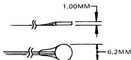
Fig. 2. Transducer size.
