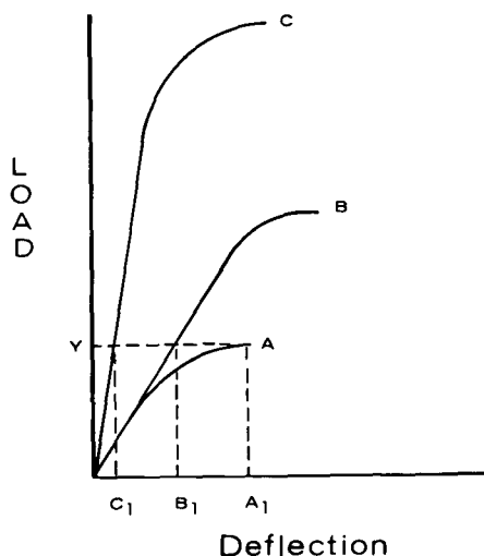
Fig. 21 A load deflection curve for same alloy round wires. Wire C has a larger diameter than wires A and B. It has greater stiffness as shown by the greater slope of its curve. Wires A and B are the same diameter hence have the same slope and stiffness. Wires A and B differ in their work hardening and heat treatment properties. Wire A is softer than wire B. With a given load, y , note the deflection characteristics of the three wires ( C_1 , B_1 , A_1 ).
