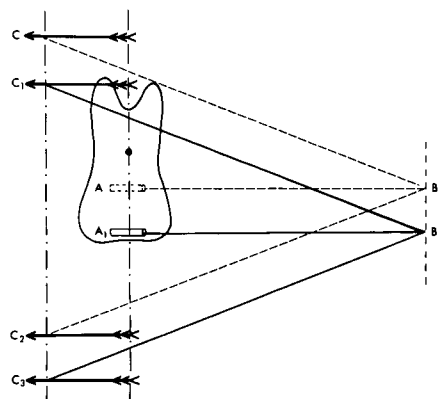
Fig. 12 Illustrates the effect of tube position variability with constant facebow design. Tube position A with facebow ABC creates more rotation or tipping than tube position A, with facebow A 1 , B 1 , C 1 ; if the same facebows were turned over then tube position and facebow A 1 , B 1 , C 1 would create the greater rotation. The outer bow should be positioned by facebow design while the headgear tube should be positioned for convenience.
