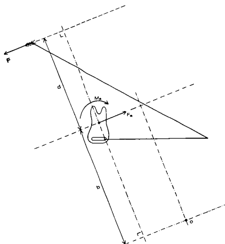
Fig. 5 In order to determine the moment in a headgear problem, choose any point (O) and determine the moments acting around it. \therefore Sum moments = F_r^b - F(d+b) = F_r^b - F^d - F^b . F_r = F . \therefore \Sigma moments = -F^d or counter-clockwise. Conclusion: Force times its perpendicular distance to the center of resistance equals the effective moment.
