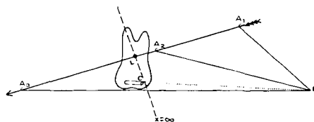
Fig. 10 Headgear facebows with varying outer bow lengths A_1 , A_2 , A_3 . All create molar translation because the resultant headgear force vector passes through the center of resistance (.). The center of rotation (X) is at infinity ( \infty ).
