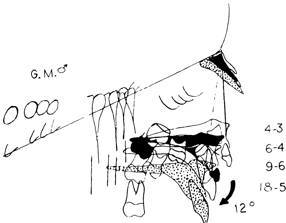
Fig. 11A Growth behavior in a male patient treated for Brodie syndrome. Treated with two stages of extraoral traction. Note 12° backward change in point A and distal movement of deciduous and permanent molars from age 4-3 to 18-5. Compare with normal growth shown in Fig. 2.
