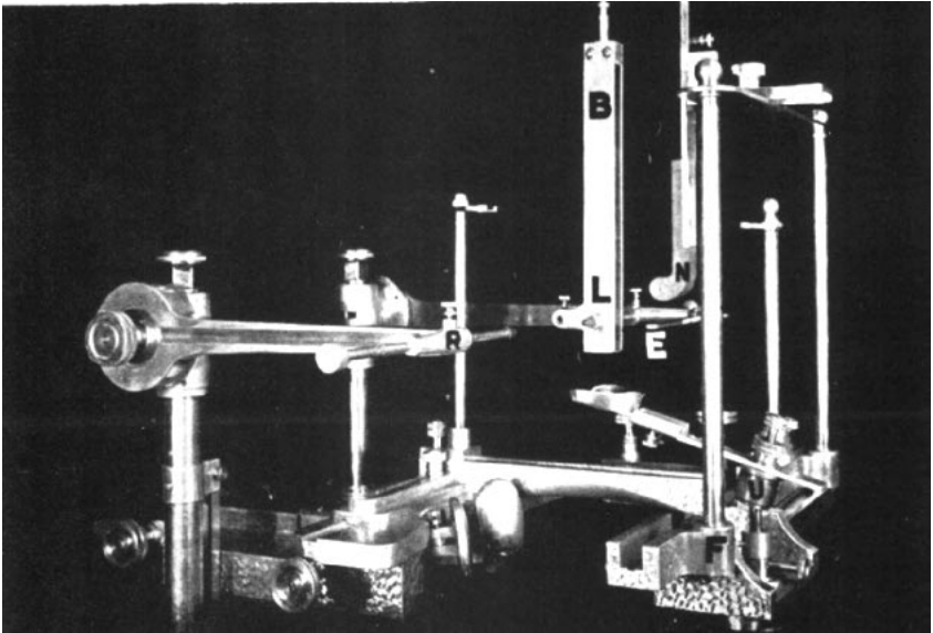
Fig. 10 The Broadbent Head Holder for roentgenographic studies of the living head. Built in the Anatomical Laboratory Western Reserve University for the Bolton Study of the development of the face of the growing child.
