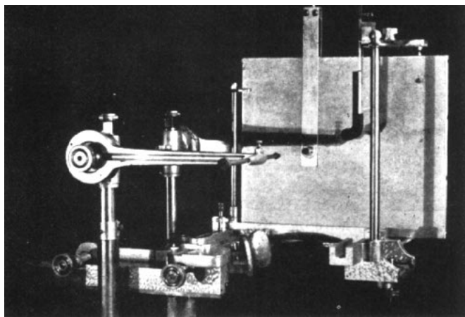
Fig. 12 The Head Holder with cassette in its place for lateral roentgenogram.
