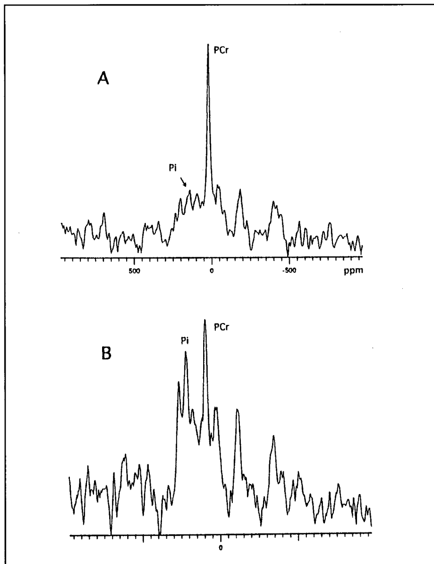
Figure 7 Phosphate-31 nuclear magnetic resonance ( ^{31}\text{P} -NMR) spectroscopy of a resting (A) and contracting (B) human masseter muscle showing dramatic changes in levels of inorganic phosphate (Pi) and phosphocreatinine (PCr) during muscle function. Metabolism of the phosphocreatinine into inorganic phosphate by the contracting muscle causes a substantial increase in the Pi:PCr ratio. Deviations from normal changes in the Pi:PCr ratios may be an indicator of aberrant muscle function such as that occurring in patients with temporomandibular disorders (courtesy of Dr. Arthur J. Miller).
