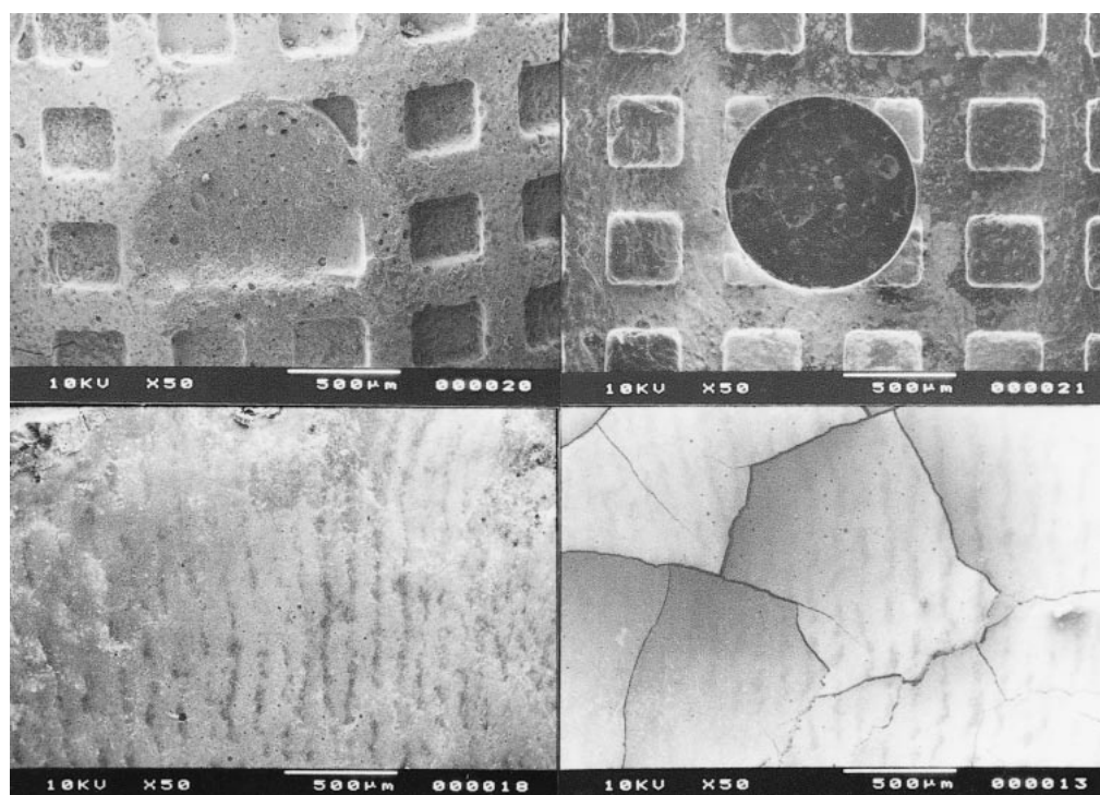
FIGURE 10. Scanning electron micrographs of typical fracture surfaces on the enamel side (left) and the bracket side (right) after shear bond test (top micrographs show cement-bracket interface failure, and bottom ones show enamel-cement interface failure).
