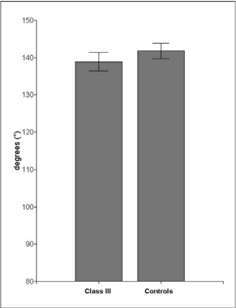
Figure 4. Distribution of \angle Ca-S-Ba broken down by group.
