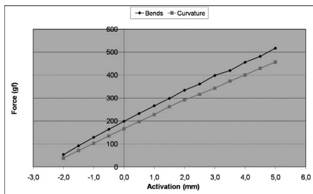
Figure 3. Horizontal force variation in the titanium T-loop springs (TTLSs) preactivated by bends and by curvature over a range of 7 mm of deactivation.
