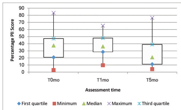
Figure 1. Distribution of PI measurements at T0mo, T1mo, and T5mo.
