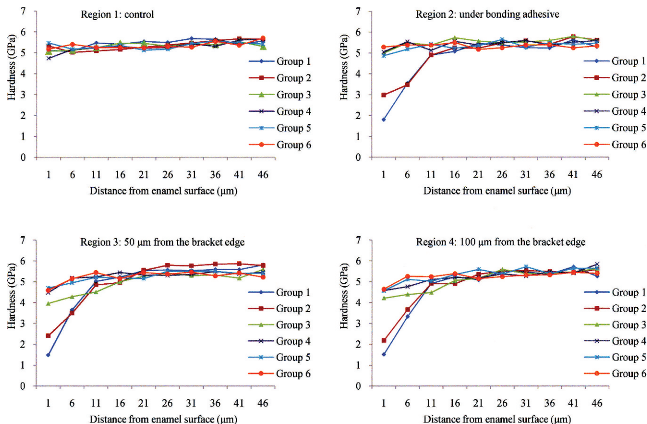
Figure 2. Mean values of hardness of enamel at different distances from the surface after immersion in demineralization solution. Group 1, Transbond XT etch-and-rinse adhesive system; group 2, Transbond Plus Color Change etch-and-rinse adhesive system; group 3, Transbond XT SEP adhesive system; group 4, Transbond Plus Color Change SEP adhesive system; group 5, Beauty Ortho Bond SEP adhesive system; and group 6, Fuji Ortho LC Automix RMGIC adhesive system.
