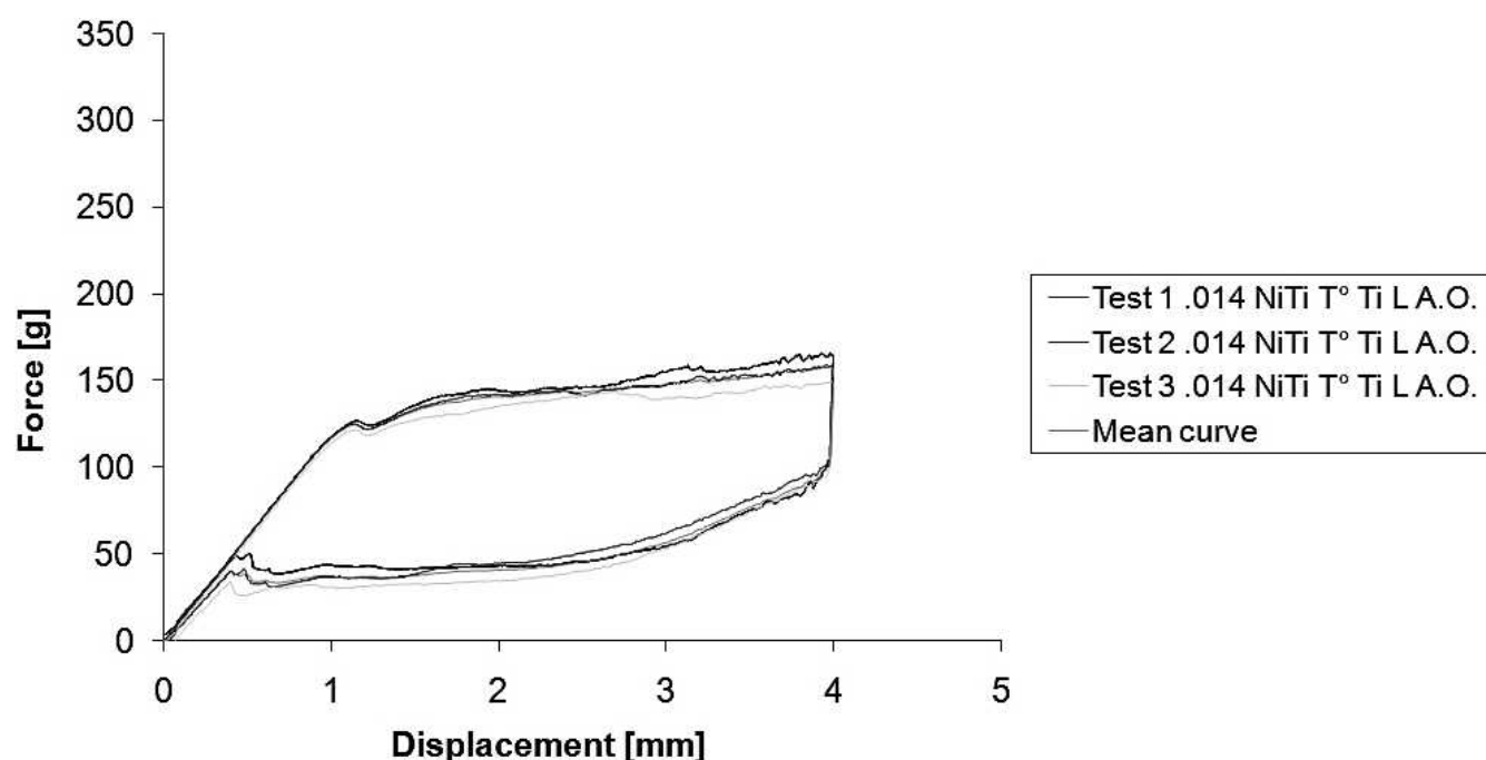
Figure 17. Load/deflection curve of 0.014 Thermo-Ti Lite (American Orthodontics).
