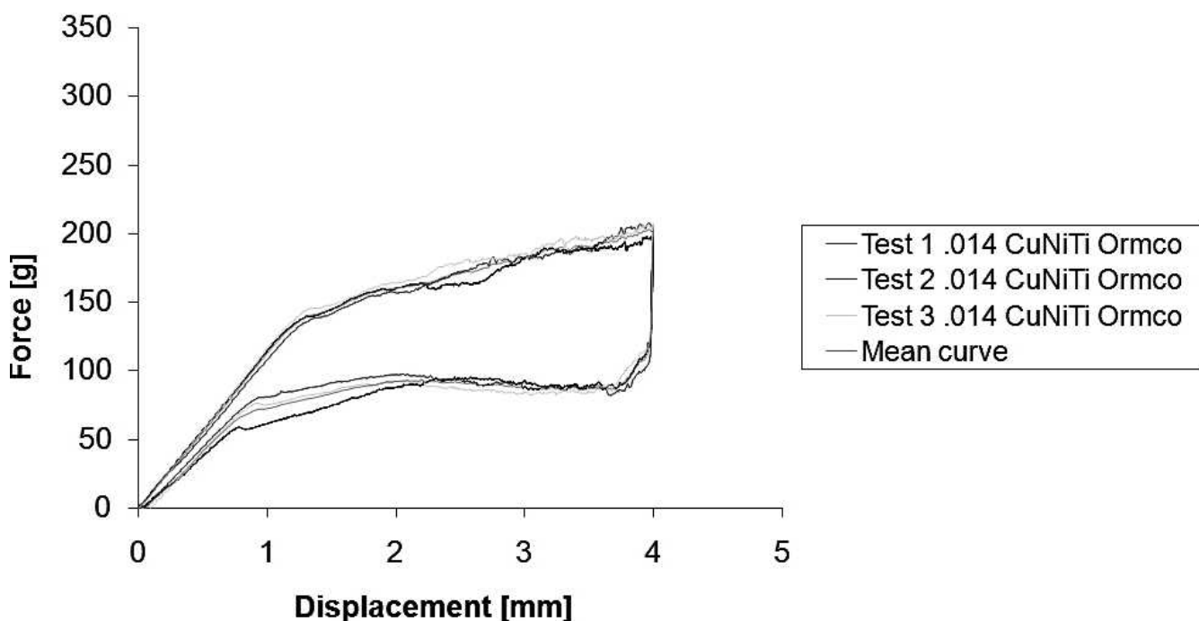
Figure 10. Load/deflection curve of 0.014 CuNiTi (Ormco).
