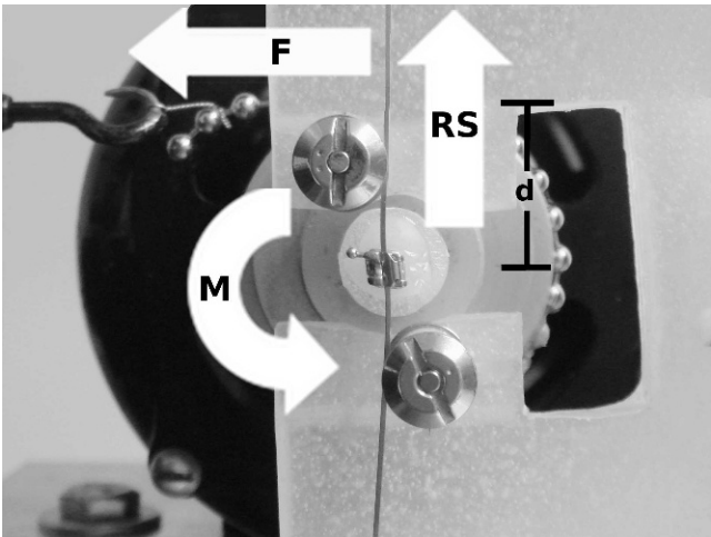
Figure 1. The bracket-archwire interface of the testing assembly as demonstrated with a 0.019×0.025" stainless steel archwire/In-OvationR bracket couple at the end of a test run. A lateral force (F) rotates the axle and mounted bracket, while the archwire is pulled vertically through the bracket by the crosshead of the Instron machine. The lateral force rotating the bracket and the force required to pull the archwire (RS) were recorded simultaneously. The moment (M) applied to the bracket was calculated as M = F \times d .
