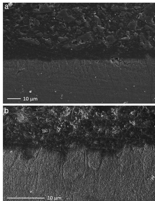
Figure 1. SEM of the interface between sound enamel and adhesive (bracket not visible) at 1000 \times (a) and 3000 \times (b) magnification.
