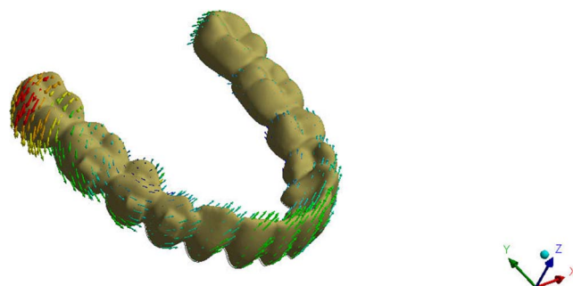
Figure 8. Aligner deformation of the ATT 4.4–4.6 3° simulation.
