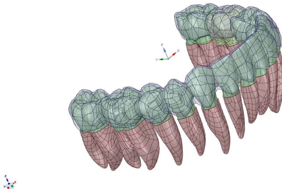
Figure 1. CAD model.
