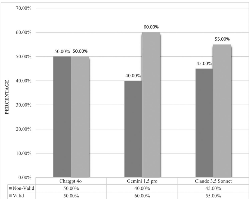
Figure 4. Analysis of valid and invalid responses in a high-threshold validity assessment.
